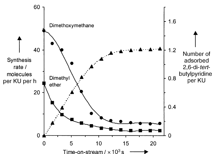
Figure 1. Adsorption uptakes ( \blacktriangle ) and rates of DMM ( \bullet ) and DME synthesis ( \blacksquare ) as a function of time-on-stream during addition of 2,6-di- tert -butylpyridine to \text{H}_5\text{PV}_2\text{Mo}_{10}\text{O}_{40}/\text{SiO}_2 ( 0.28 \text{ KU nm}^{-2} , 453 K, 4 kPa \text{CH}_3\text{OH} , 9 kPa \text{O}_2 , \text{CH}_3\text{OH}/2,6\text{-di-}t\text{-butylpyridine (mol)} = 1110/1 ).
