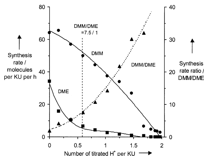
Figure 3. Rates of DMM ( \bullet ) and DME synthesis ( \blacksquare ) and their ratios of DMM/DME ( \blacktriangle ) as a function of the number of protons (per KU) titrated with pyridine on \text{H}_5\text{PV}_2\text{Mo}_{10}\text{O}_{40}/\text{SiO}_2 ( 0.1 \text{ KU nm}^{-2} , 453 K, 4 kPa \text{CH}_3\text{OH} , 9 kPa \text{O}_2 , \text{CH}_3\text{OH/pyridine (mol)} = 800/1 ).
