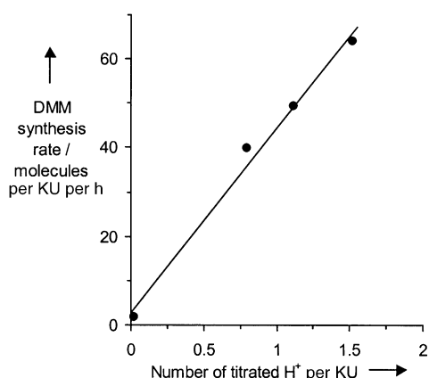
Figure 2. Rates of DMM synthesis as a function of the number of protons (per KU) titrated with 2,6-di- tert -butylpyridine on unsupported and \text{SiO}_2 -supported ( 0.1\text{--}0.65 \text{ KU nm}^{-2} ) \text{H}_5\text{PV}_2\text{Mo}_{10}\text{O}_{40} (453 K, 4 kPa \text{CH}_3\text{OH} , 9 kPa \text{O}_2 , \text{CH}_3\text{OH}/2,6\text{-di-}t\text{-butylpyridine (mol)} = 1110/1 ).
