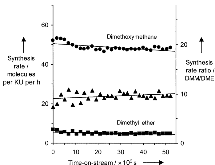
Figure 4. Rates of DMM (●) and DME synthesis (■) and their ratios of DMM/DME (▲) as a function of time-on-stream after titration of 0.6 \text{H}^+ per KU and stop of pyridine injection on \text{H}_5\text{PV}_2\text{Mo}_{10}\text{O}_{40}/\text{SiO}_2 ( 0.1 \text{ KU nm}^{-2} , 453 K, 4 kPa \text{CH}_3\text{OH} , 9 kPa \text{O}_2 , \text{CH}_3\text{OH}/\text{pyridine} (mol) = 800/1).
